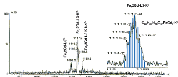
Figure 3. Electrospray mass spectrum of Fe,2Gd-3L3. The calculated (blue) and experimental (black) isotopic distributions of the molecular ion are shown in the expanded region.
