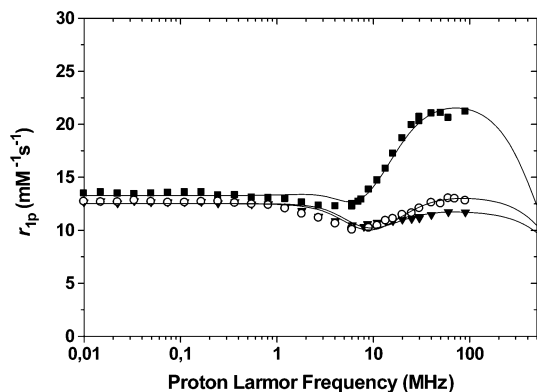
Figure 4. 1/T_1 NMRD profile at 298 K and pH 7.4 of Fe,Gd-L A (▼), Fe,-Gd-3L B (○), and Fe,2Gd-3L C (■). Longitudinal relaxivities are given per Gd(III) ion.
